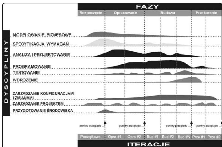
Rysunek 2.1. Rational Unified Process
