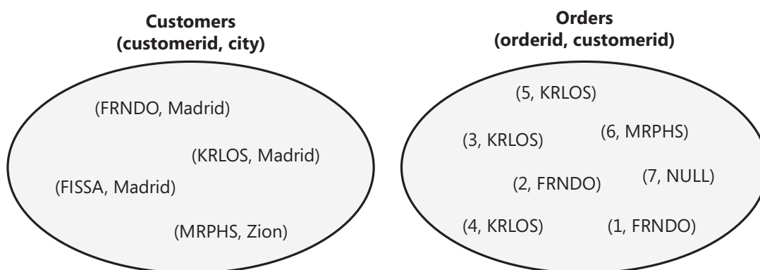
RYСУNEK 1-2 Zbiory Customers oraz Orders.
