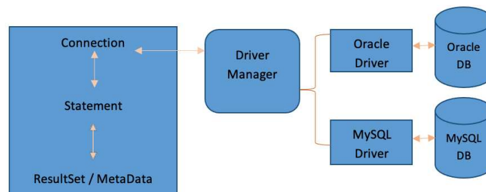
Figure 1.2: Core components of JDBC API
