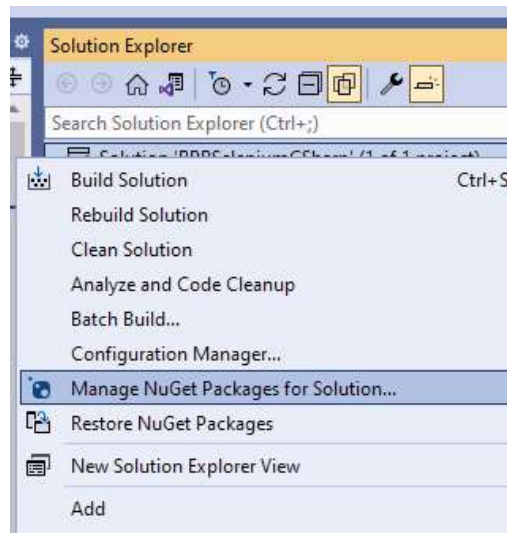
Figure 1.9: NuGet Packages
