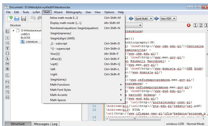
TeXmaker
