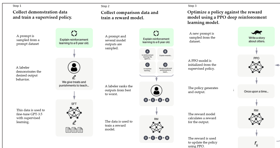
Figure 1.1: Training ChatGPT
