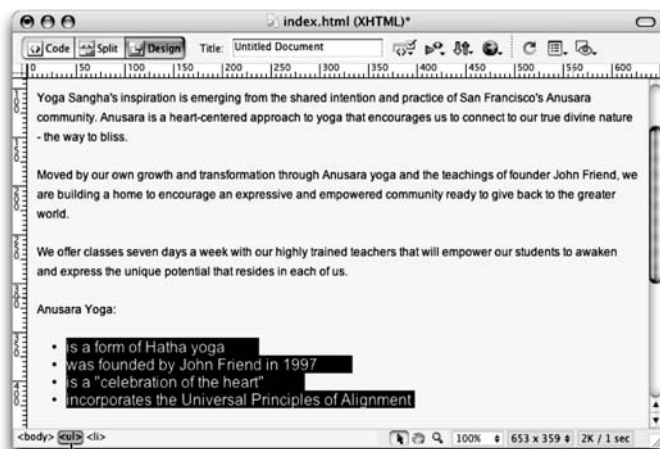
Tag selector
