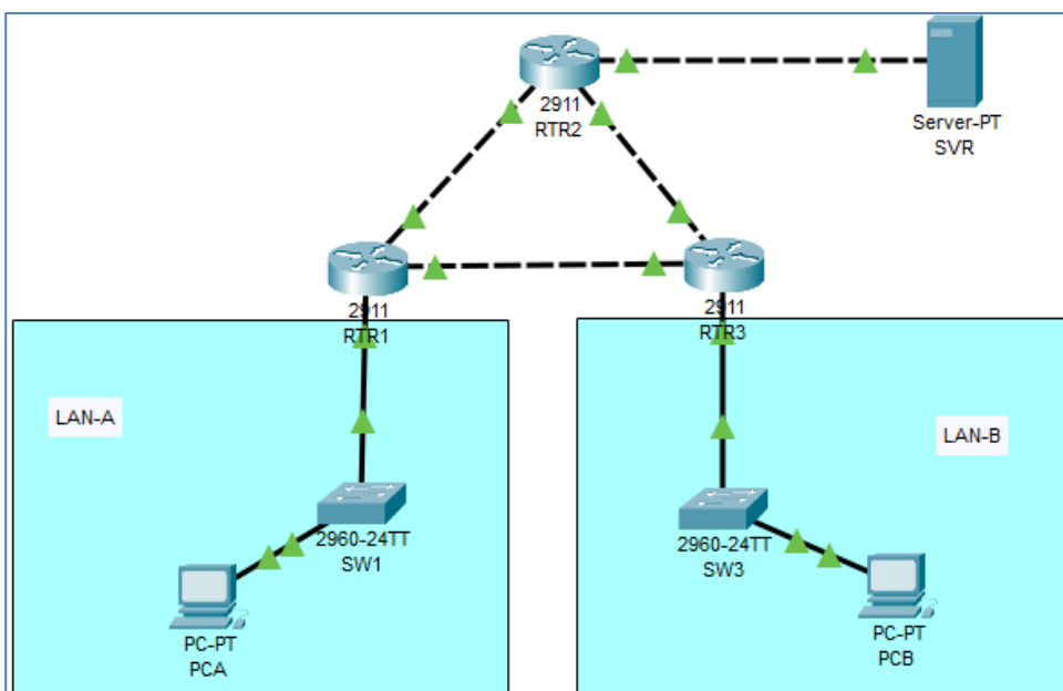
Figure 13.11 Network topology
