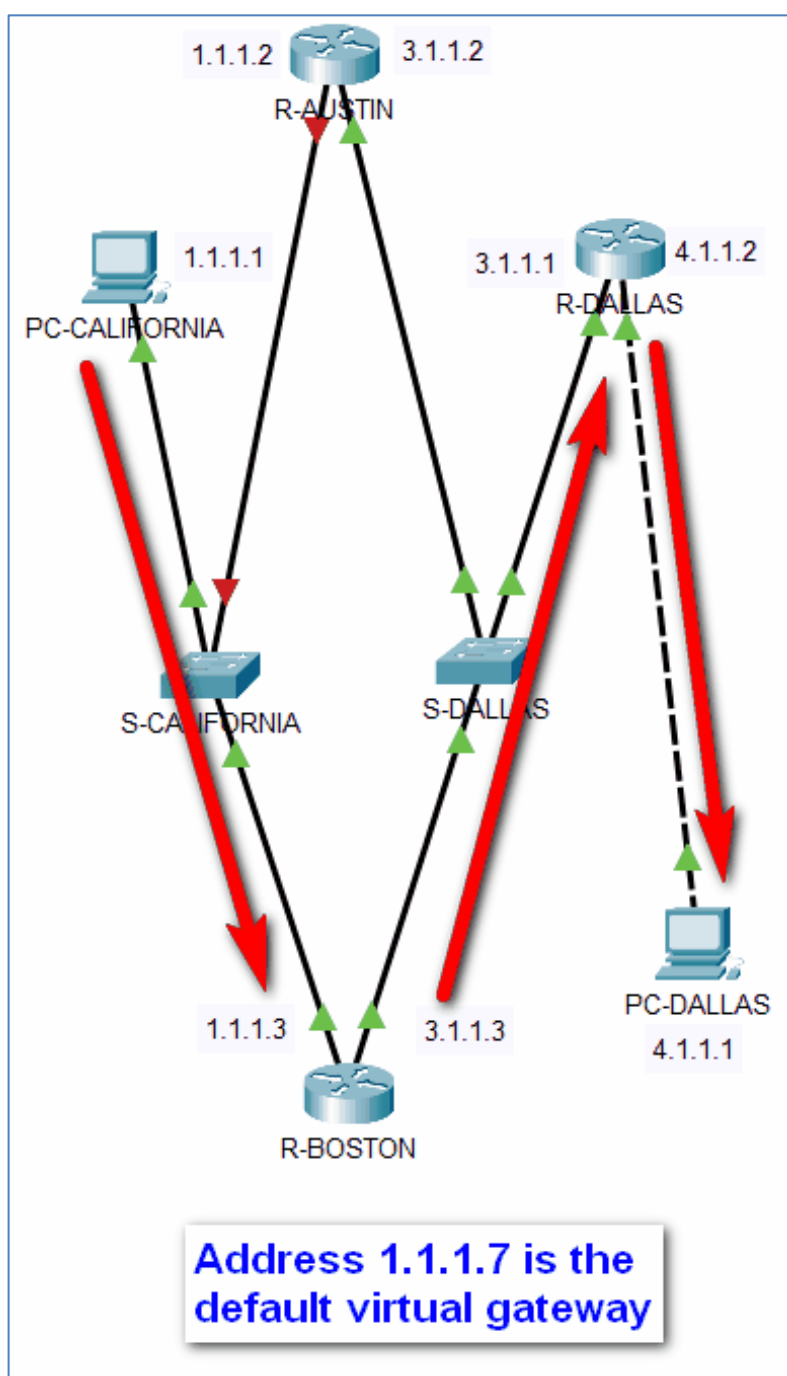
Figure 13.9 Route in case of R-AUSTIN failure
