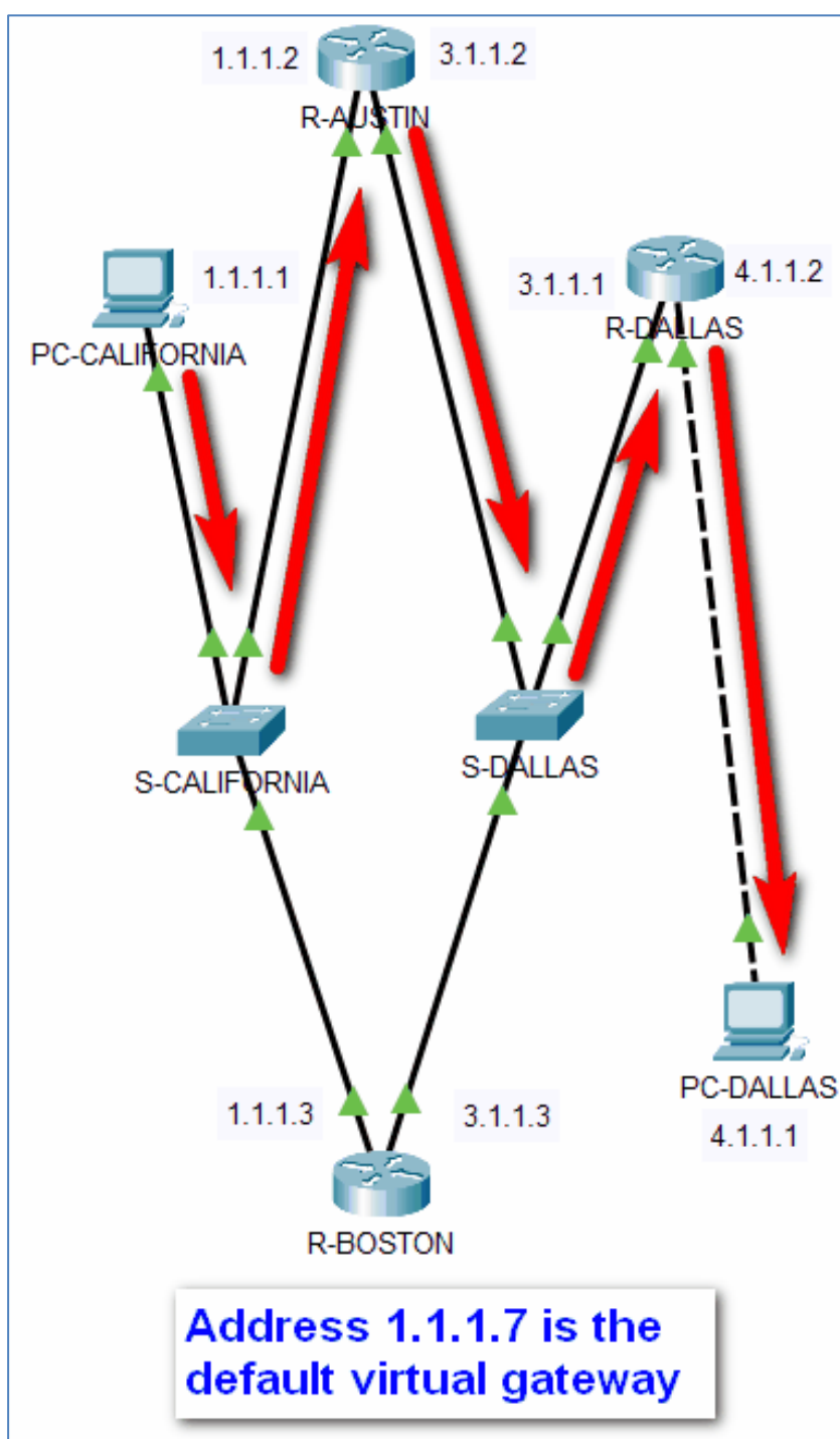
Figure 13.10 Route in case of failure R-BOSTON
