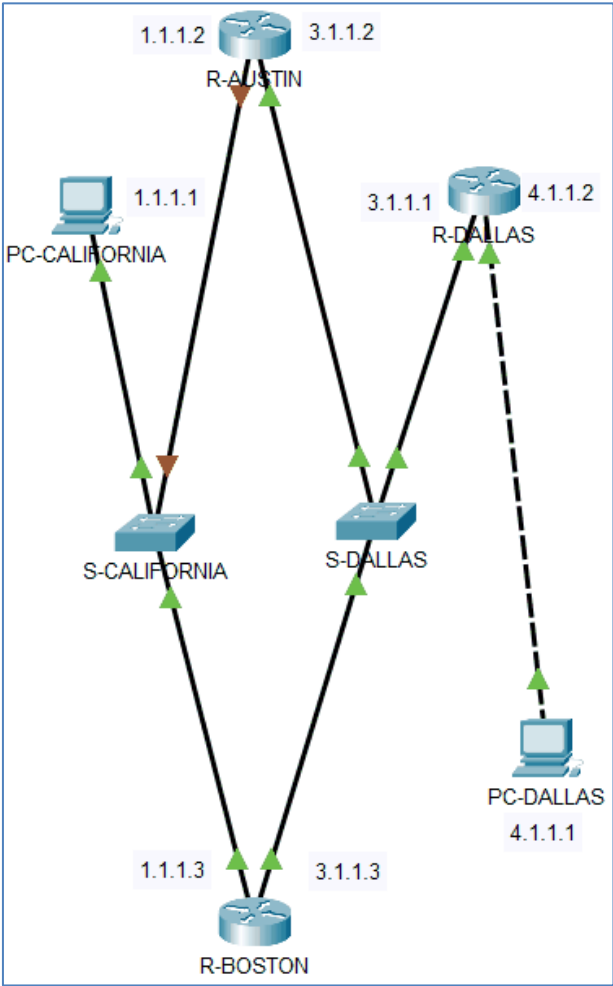
Figure 13.3 Network topology with Fa0/0 interface failure in R-AUSTIN
