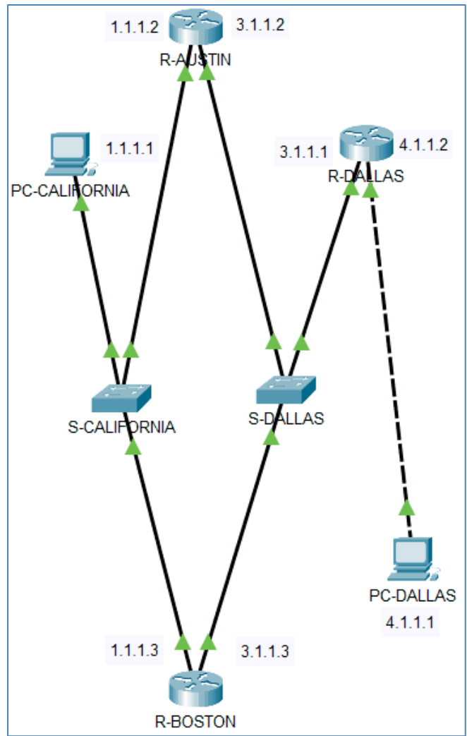
Figure 13.1 Network topology
