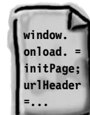
validation.js
