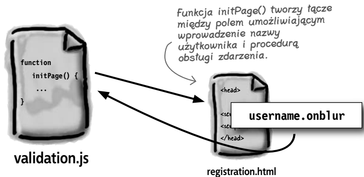
registration.html
